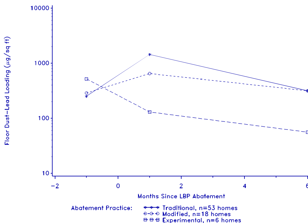
Figure 3-7. Geometric mean floor dust-lead loading ( \mu\text{g}/\text{ft}^2 ) post-abatement by abatement practice performed (Baltimore “Traditional”/“Modified” and Experimental Practices Studies).
